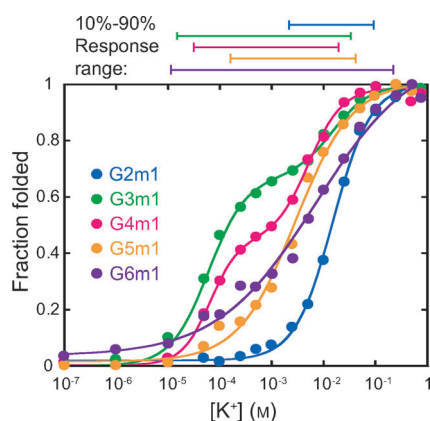
Figure 3. Graph of the fraction of G2m1–G6m1 QGSs folded at 262 nm by CD spectroscopy. G3m1 and G4m1 were fit to a three-state equation (Equation S2), while G2m1, G5m1, and G6m1 were fit to a two-state equation (Equation S1). The response range for each QGS is defined from 10–90% folded and is depicted with bars of matching color above the panel. The K_{1/2}^+ and n values are in Table 1. See Figure S2 and S7–S12 for full CD spectra and individual fits.
